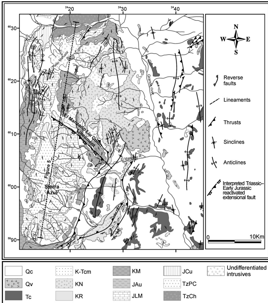
Fig. 4. Geologic map of Sierra Azul and western Sierra de Palauco region, modified from Groeber, 1937; Dessanti, 1973; Legarreta et al., 1985; Kozlowski et al., 1989; Gulisano and Gutierrez Pleimling, 1994; Dicarlo, 2005. Qc, clastic Quaternary; Qv, volcanic Quaternary; Tc, Tertiary; K-Tcm, Malargüe Group; KN, Neuquén Group; KR, Rayoso Group; KM, Mendoza Group; JAu, Auquillo Formation; JLM, La Manga Formation; JCu, Cuyo Group; TzPC, pre-Cuyo Group; TzCh, Choiyoi Group.
