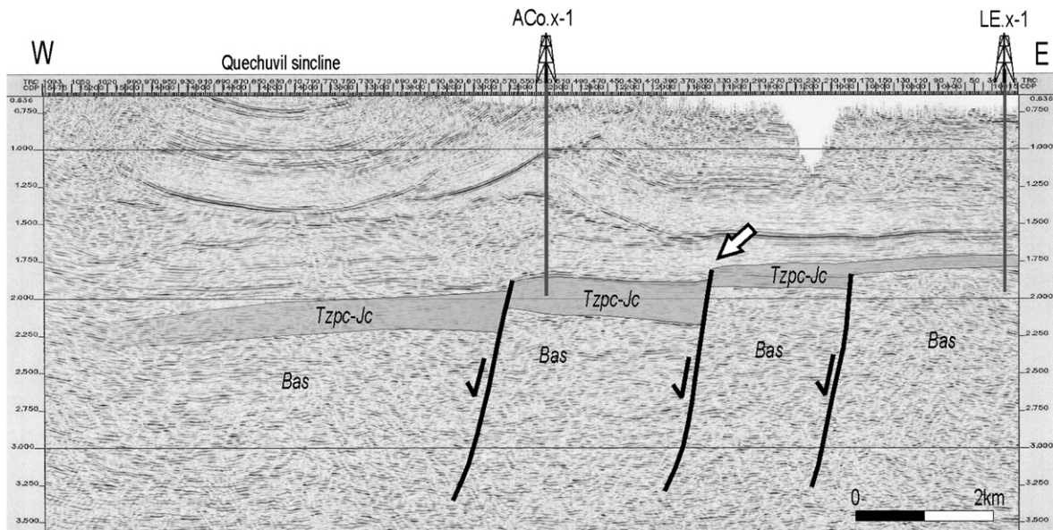
Fig. 6. Seismic line used to build the structural section in Fig. 7b. The arrow indicates the normal fault highlighted in Fig. 2. Bas, basement of the Mesozoic succession (Choiyoi Group); Tzpc, pre-Cuyo Group; Jc, Cuyo Group. ACo.x-1: Arroyo Coehueco x-1. LE.x-1: Loma de las Espinas x-1. See Fig. 2 for location.
